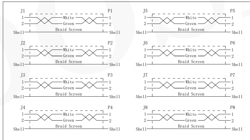
*Wiring Table
