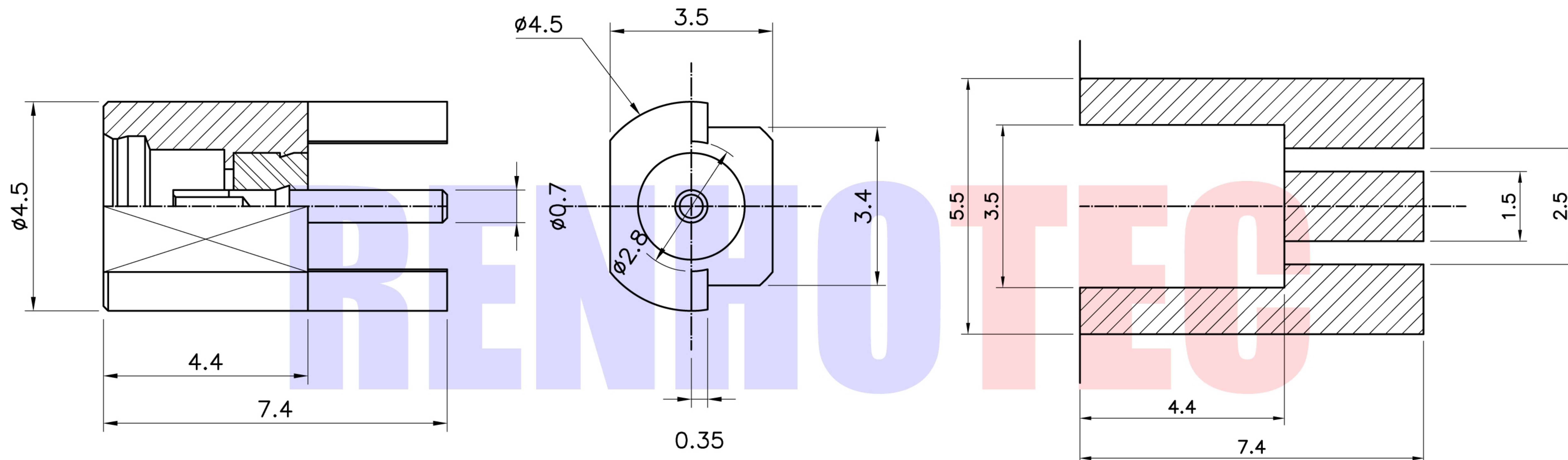
SOLDERPAD LAYOUT
